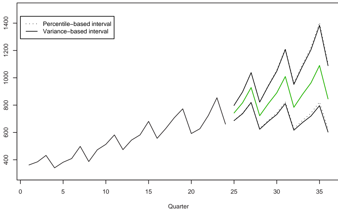
Figure 2: Quarterly sales data with three years of forecasts. The solid lines show prediction intervals calculated as \mu_h \pm 1.96\sqrt{\hat{v}_h} and the dotted lines show prediction intervals computed by generating 20,000 future sample paths from the fitted model and finding the 2.5% and 97.5% quantiles at each forecast horizon.
