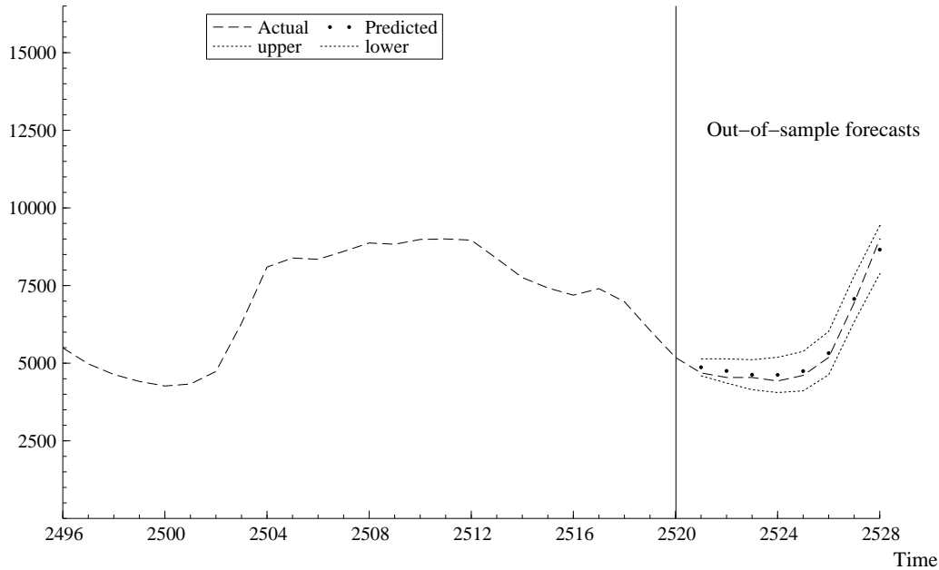
Fig. 5. MS(2; 24, 168) Restriction 3: Point forecasts and 80% prediction intervals for the first 8 hours in the next week ( t = 2521, \dots, 2528 ) of the utility demand.
