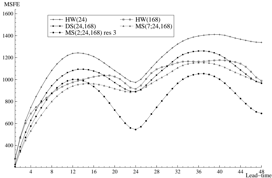
Fig. 4. Forecasting accuracy (MSFE) for lead-times from 1 to 48 hours (i.e. 2 days)
