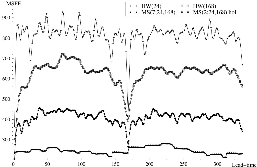
Fig. 7. Forecasting accuracy (MSFE) for lead-times from 1 to 336 hours (i.e. 2 weeks)
