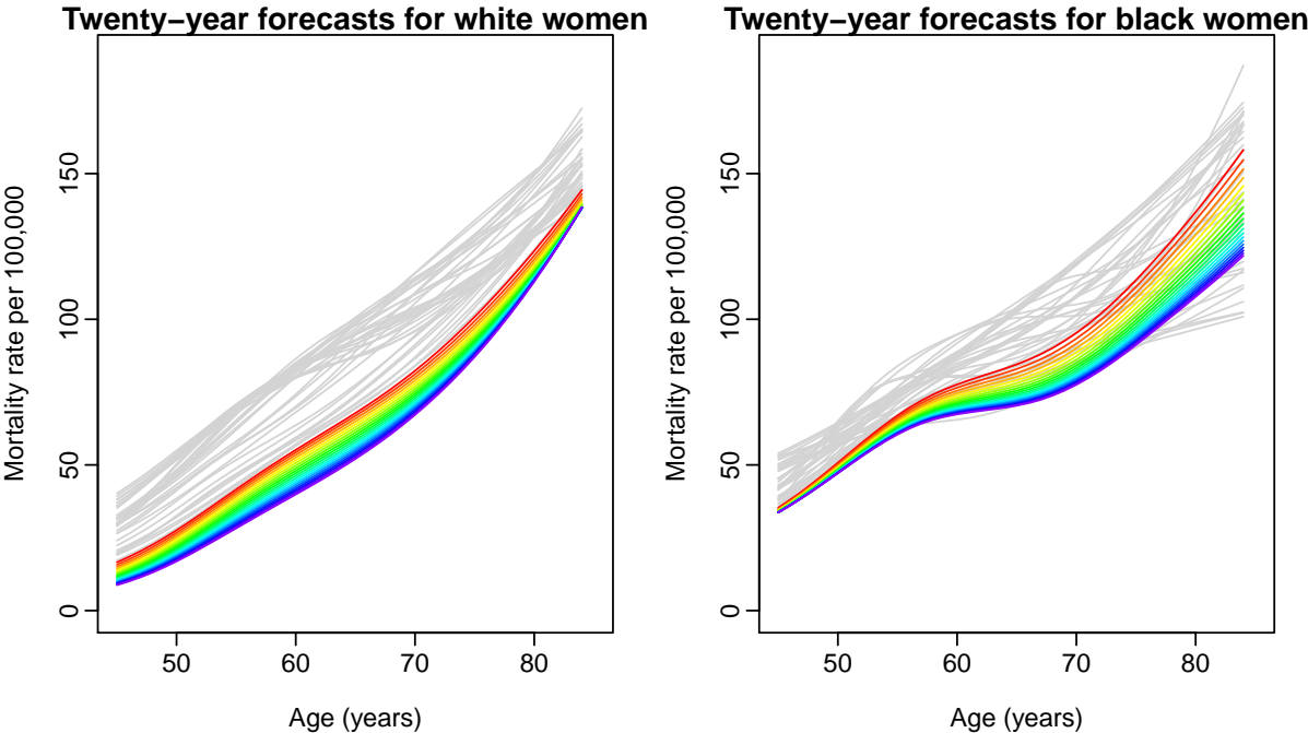
Figure 4: Twenty-year forecasts (2005–2024) for breast cancer mortality rates for white women and black women. The years are plotted in “rainbow” order with the later years in violet. The gray curves show the smoothed historical data from 1969 to 2004.
