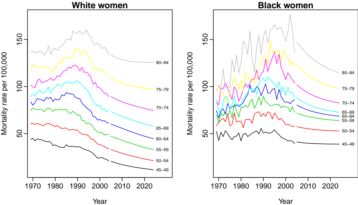
Figure 5: Historical data and twenty-year forecasts (2005–2024) for breast cancer mortality rates for white women and black women by age-group. The break in the lines indicates the end of the historical data and the start of the forecasts.
