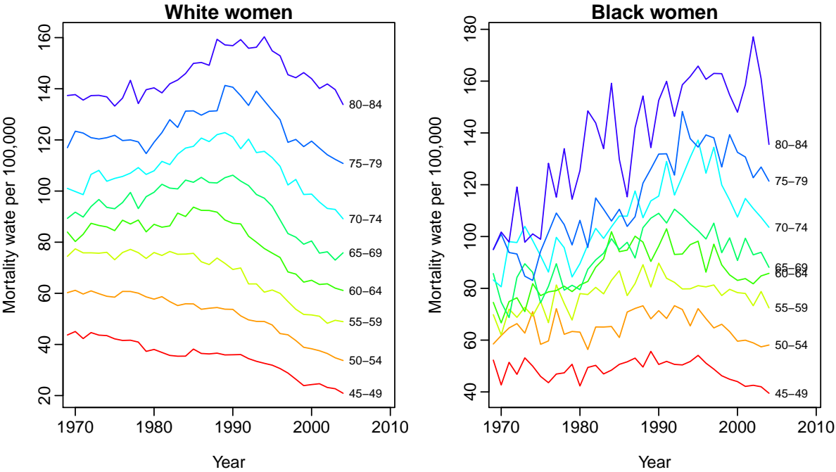
Figure 1: Breast cancer mortality rates (per 100 000 women) by age-group among white and black US women (1969–2004).
