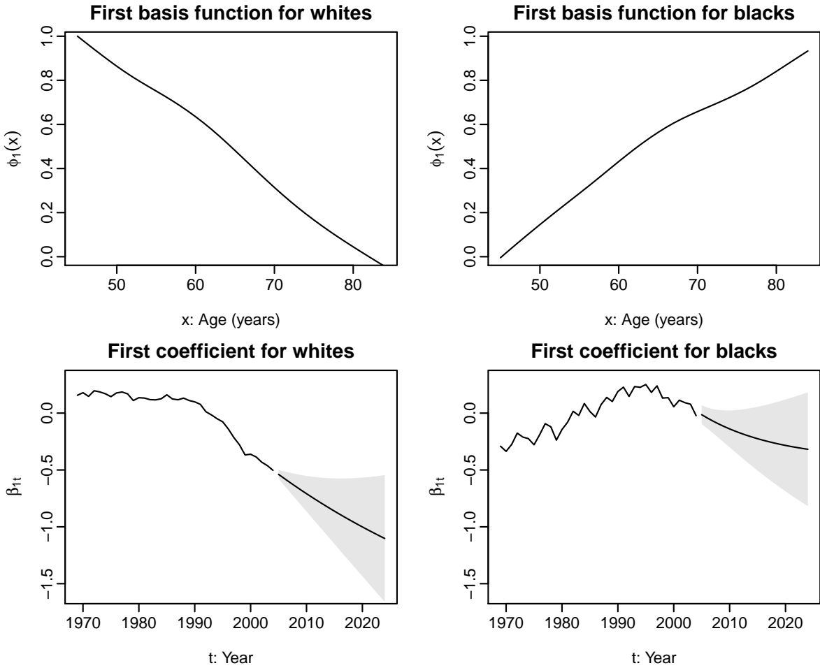
Figure 3: The first basis functions and the first coefficients from the models for white and black women. Twenty-year forecasts are also shown for the first coefficients of each model.
