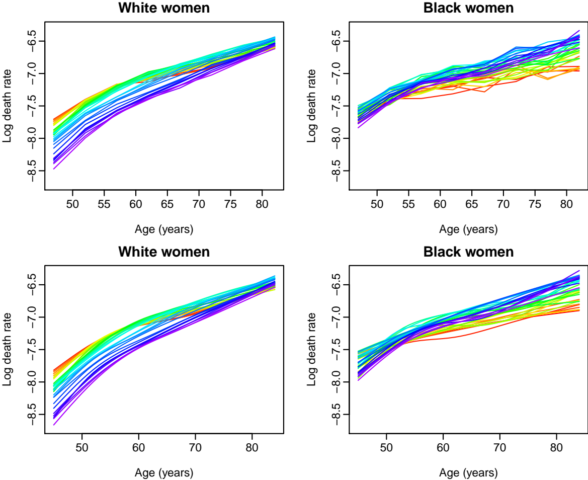
Figure 2: Log mortality rates for white and black US women (1969–2004). In the upper panel original log rates are plotted whereas in the lower panel, log rates after smoothing are plotted. Penalized regression splines are used to smooth the data. The curves are ordered in time using rainbow colors. The oldest data (from 1969) are shown in red, with the most recent data (from 2004) shown in purple.
