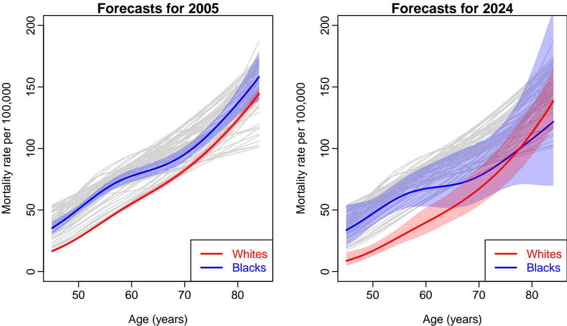
Figure 6: Forecast (for 2005 and 2024) for breast cancer mortality rates along with 80% prediction intervals for white women and black women. The gray curves show the smoothed historical data from 1969 to 2004.
